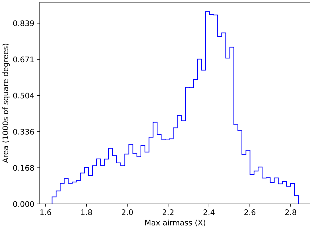
too_elab_r64_d2_gz_v3.4_10yrs WFD r band: Max airmass
