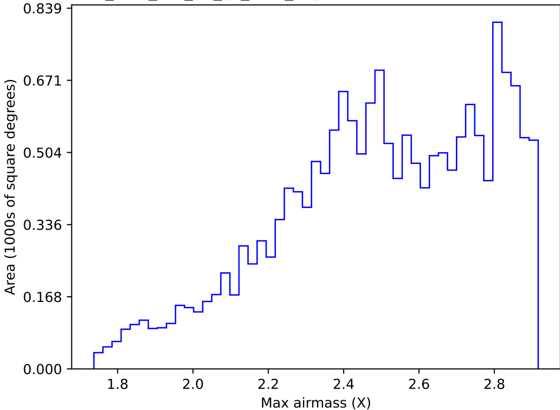
too_elab_r64_d2_gz_v3.4_10yrs WFD i band: Max airmass
