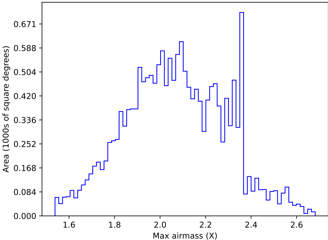
too_elab_r64_d2_gz_v3.4_10yrs WFD g band: Max airmass
