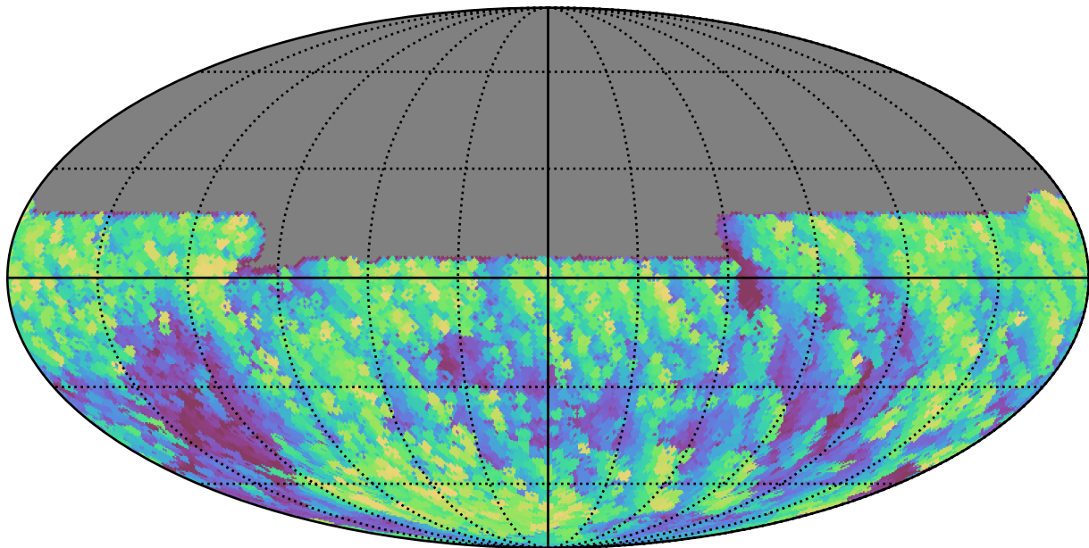
too_elab_r64_d2_gz_v3.4_10yrs All sky y band: Max airmass
