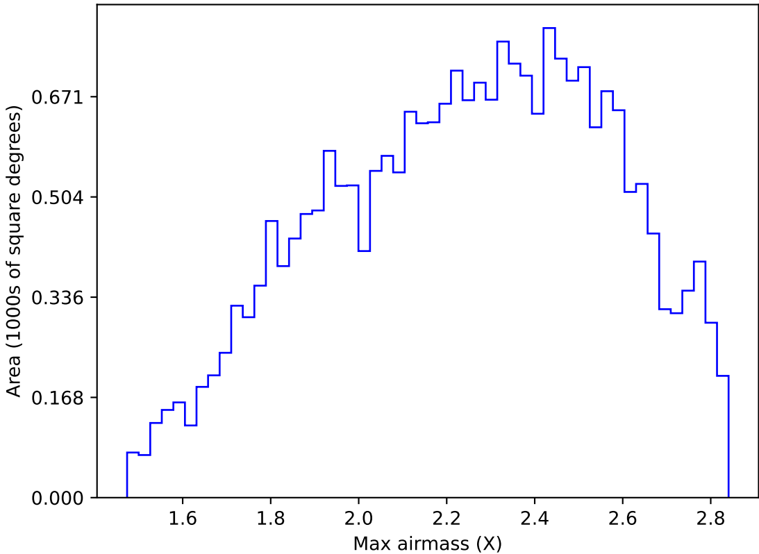
too_elab_r64_d2_gz_v3.4_10yrs All sky y band: Max airmass
