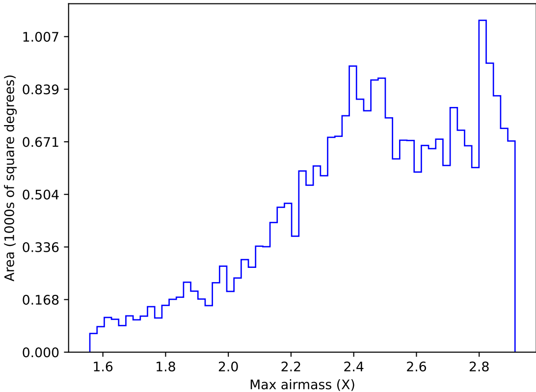
too_elab_r64_d2_gz_v3.4_10yrs All sky i band: Max airmass
