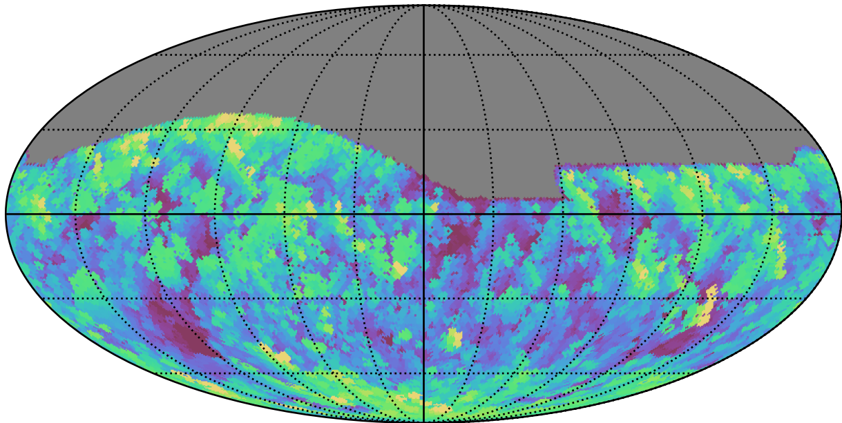
too_elab_r64_d2_gz_v3.4_10yrs All sky g band: Max airmass
