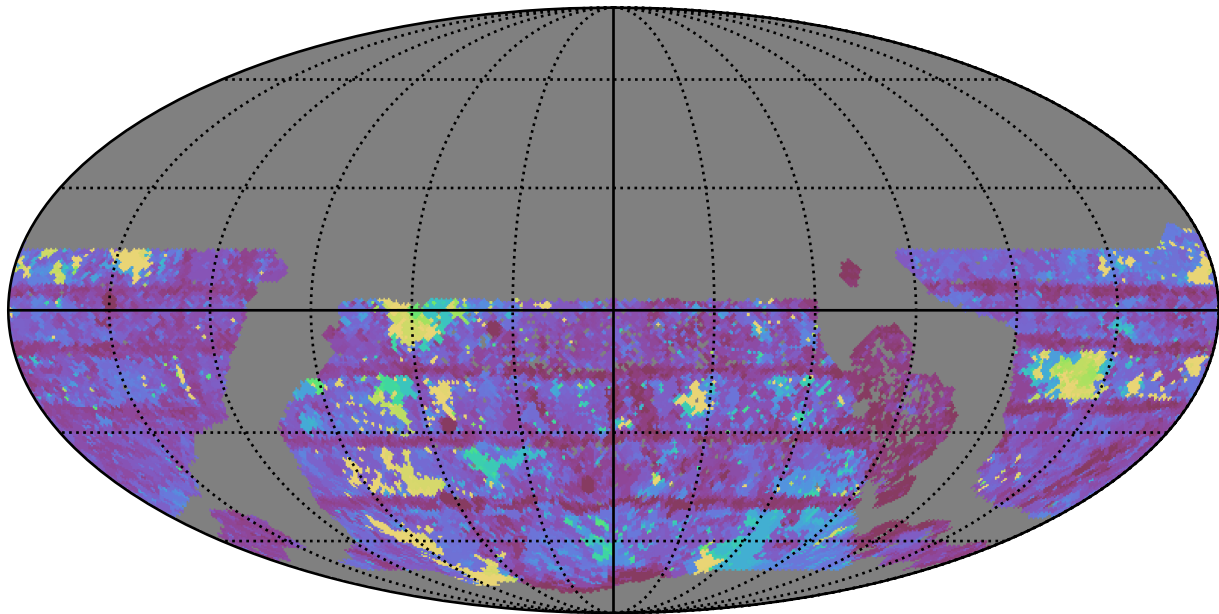
too_elab_r64_d2_gz_v3.4_10yrs WFD z band: Max Inter-Night Gap
