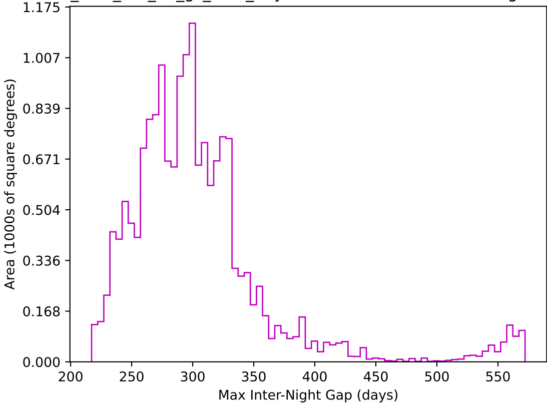
too_elab_r64_d2_gz_v3.4_10yrs WFD z band: Max Inter-Night Gap
