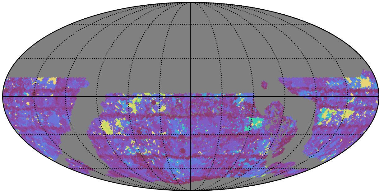
too_elab_r64_d2_gz_v3.4_10yrs WFD y band: Max Inter-Night Gap
