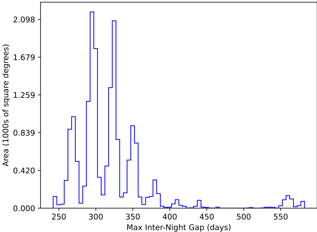
too_elab_r64_d2_gz_v3.4_10yrs WFD y band: Max Inter-Night Gap
