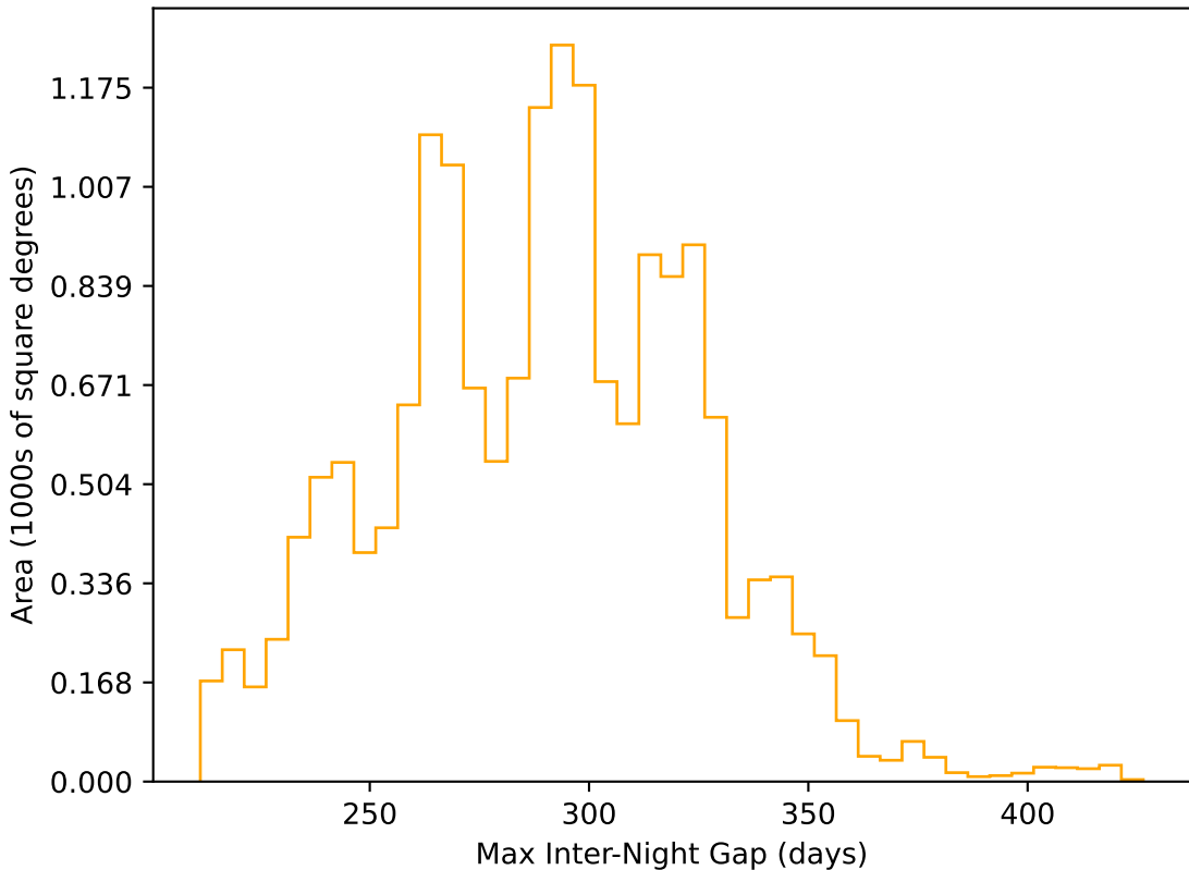
too_elab_r64_d2_gz_v3.4_10yrs WFD r band: Max Inter-Night Gap
