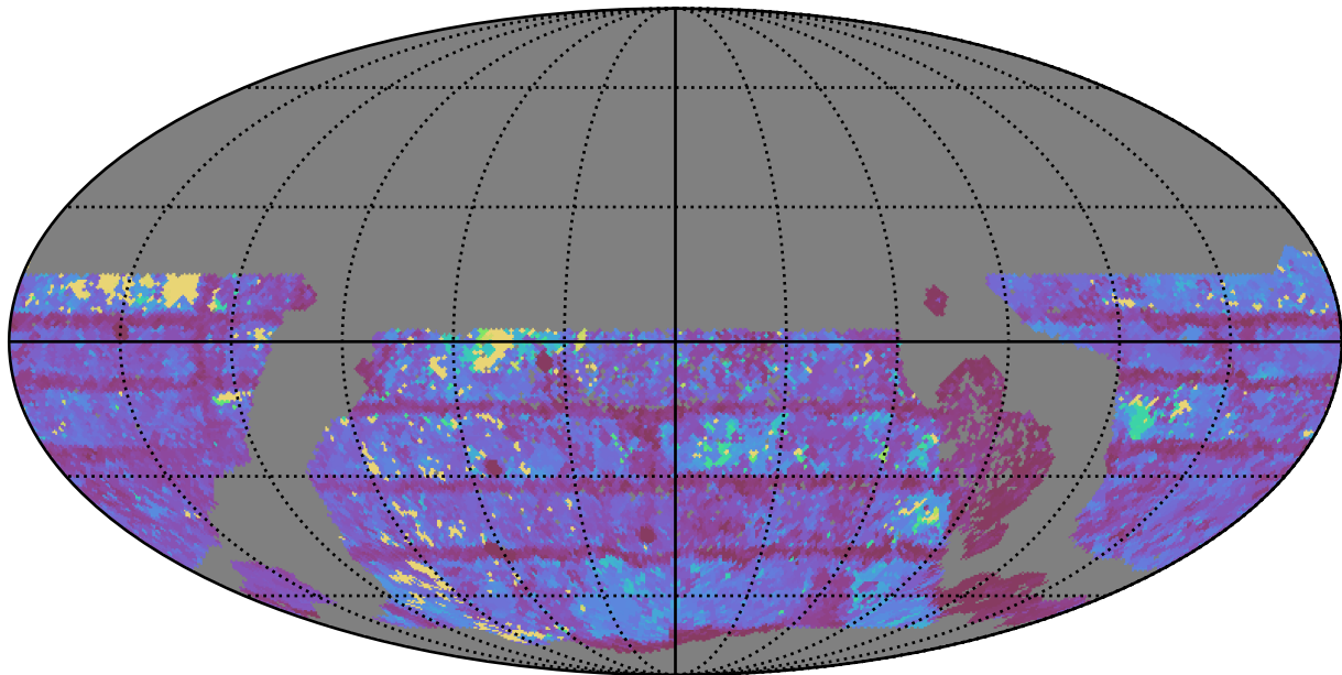
too_elab_r64_d2_gz_v3.4_10yrs WFD i band: Max Inter-Night Gap
