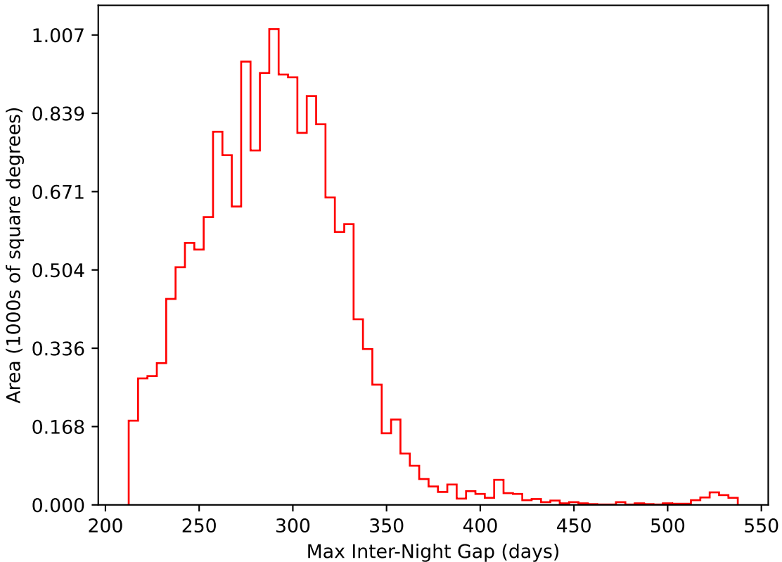
too_elab_r64_d2_gz_v3.4_10yrs WFD i band: Max Inter-Night Gap
