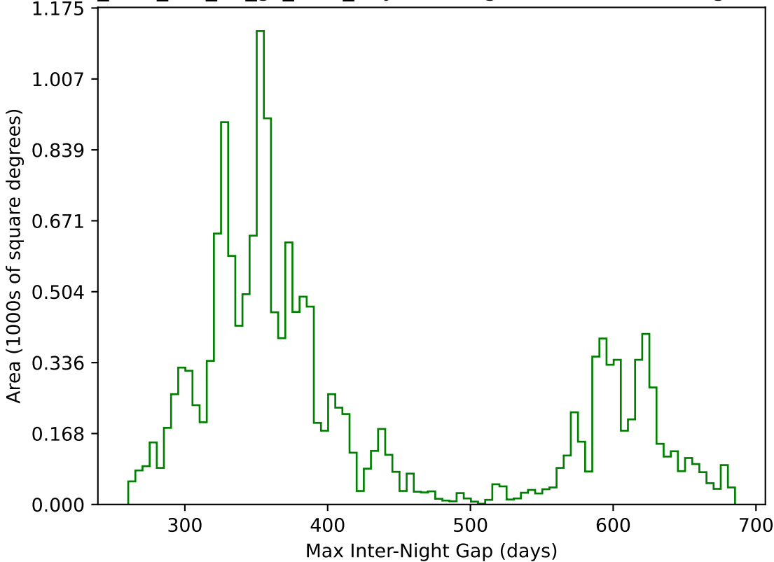
too_elab_r64_d2_gz_v3.4_10yrs WFD g band: Max Inter-Night Gap
