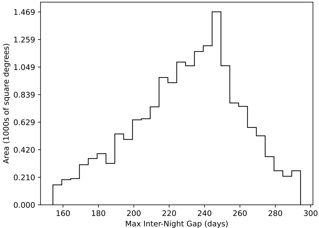
too_elab_r64_d2_gz_v3.4_10yrs WFD all bands: Max Inter-Night Gap
