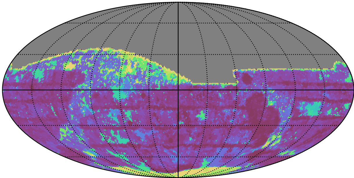
too_elab_r64_d2_gz_v3.4_10yrs All sky z band: Max Inter-Night Gap
