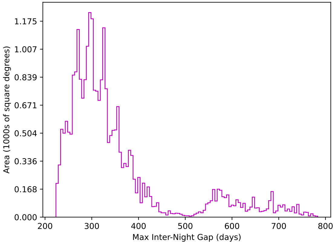
too_elab_r64_d2_gz_v3.4_10yrs All sky z band: Max Inter-Night Gap
