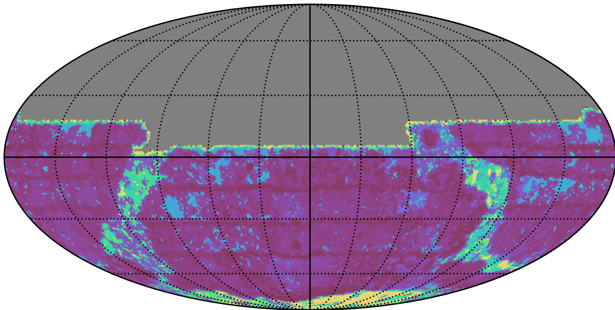
too_elab_r64_d2_gz_v3.4_10yrs All sky y band: Max Inter-Night Gap
