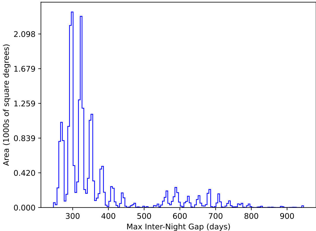
too_elab_r64_d2_gz_v3.4_10yrs All sky y band: Max Inter-Night Gap
