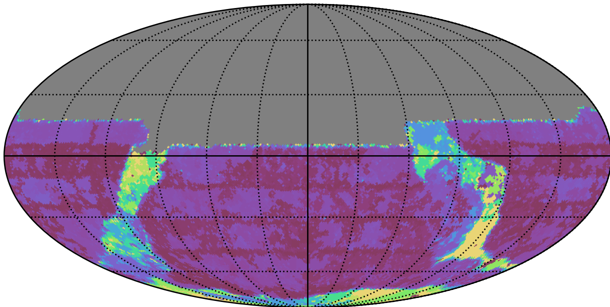
too_elab_r64_d2_gz_v3.4_10yrs All sky u band: Max Inter-Night Gap
