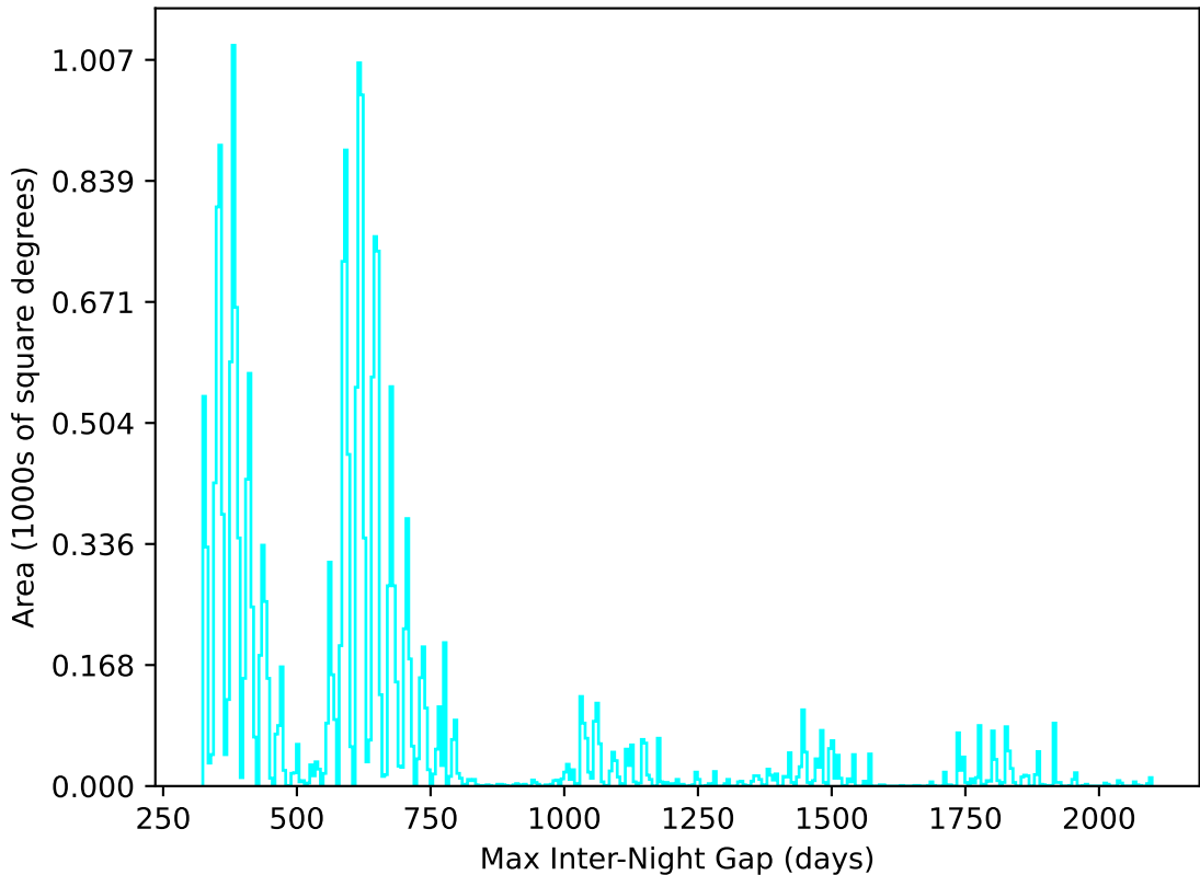
too_elab_r64_d2_gz_v3.4_10yrs All sky u band: Max Inter-Night Gap
