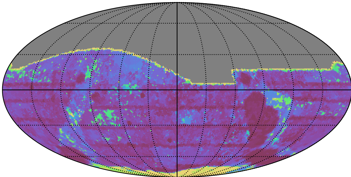
too_elab_r64_d2_gz_v3.4_10yrs All sky r band: Max Inter-Night Gap
