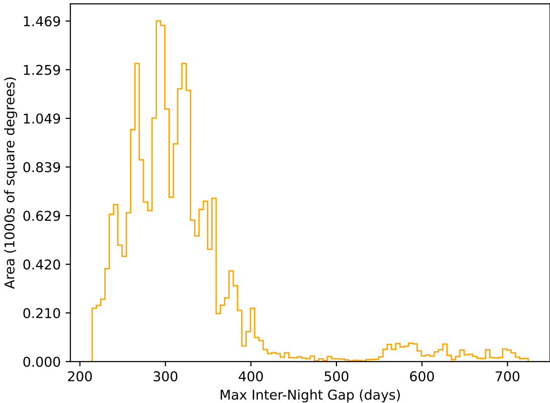
too_elab_r64_d2_gz_v3.4_10yrs All sky r band: Max Inter-Night Gap
