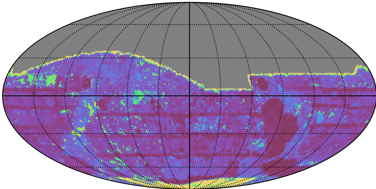
too_elab_r64_d2_gz_v3.4_10yrs All sky i band: Max Inter-Night Gap
