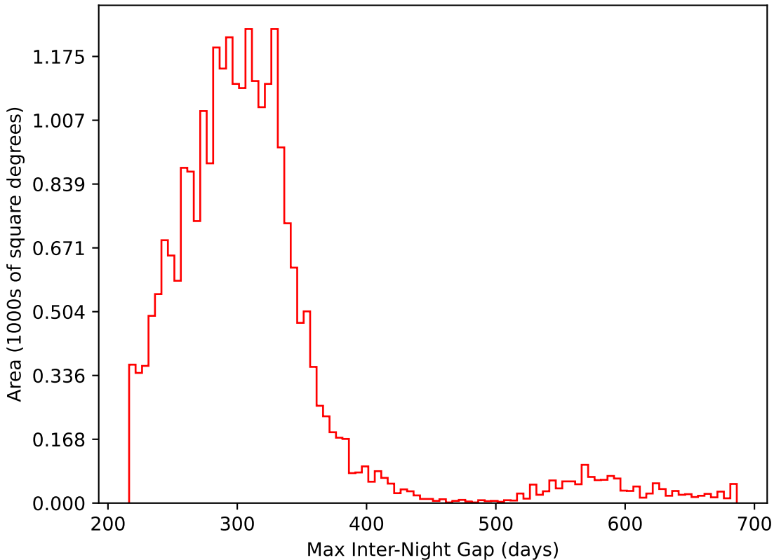
too_elab_r64_d2_gz_v3.4_10yrs All sky i band: Max Inter-Night Gap
