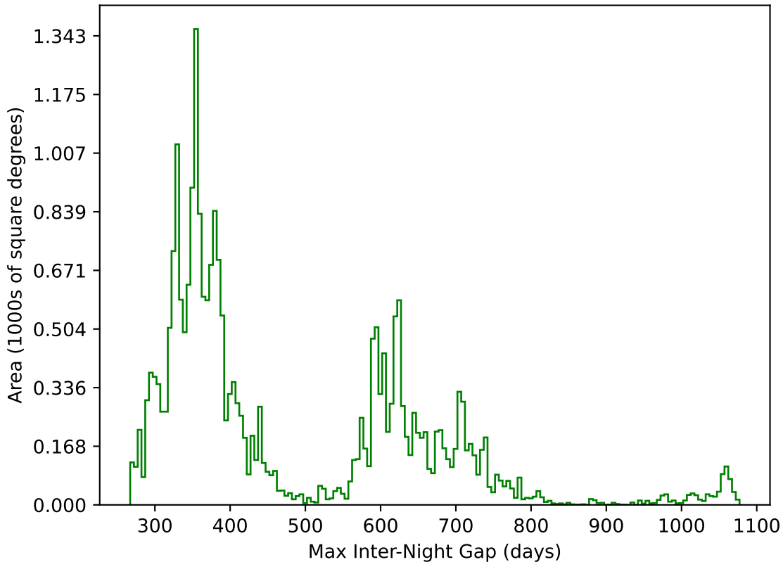
too_elab_r64_d2_gz_v3.4_10yrs All sky g band: Max Inter-Night Gap
