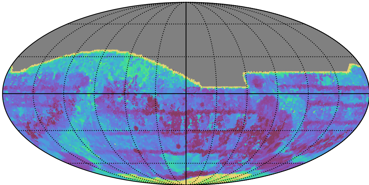
too_elab_r64_d2_gz_v3.4_10yrs All sky all bands: Max Inter-Night Gap
