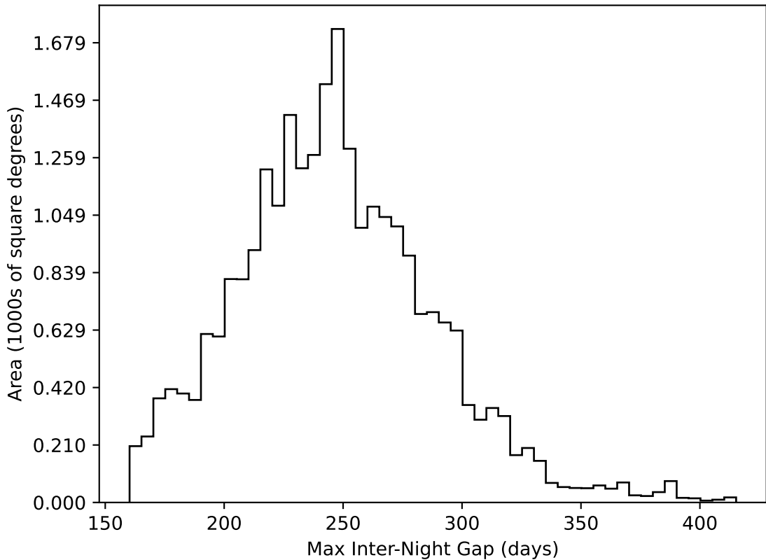
too_elab_r64_d2_gz_v3.4_10yrs All sky all bands: Max Inter-Night Gap
