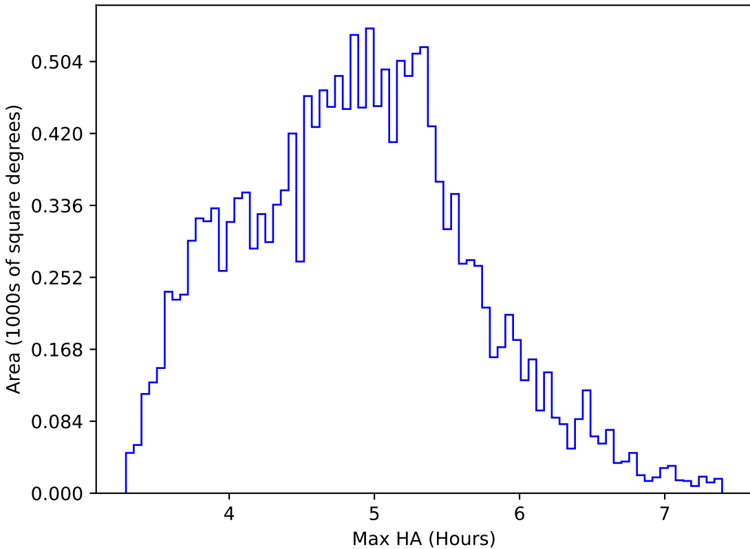
too_elab_r64_d2_gz_v3.4_10yrs WFD z band: Max HA
