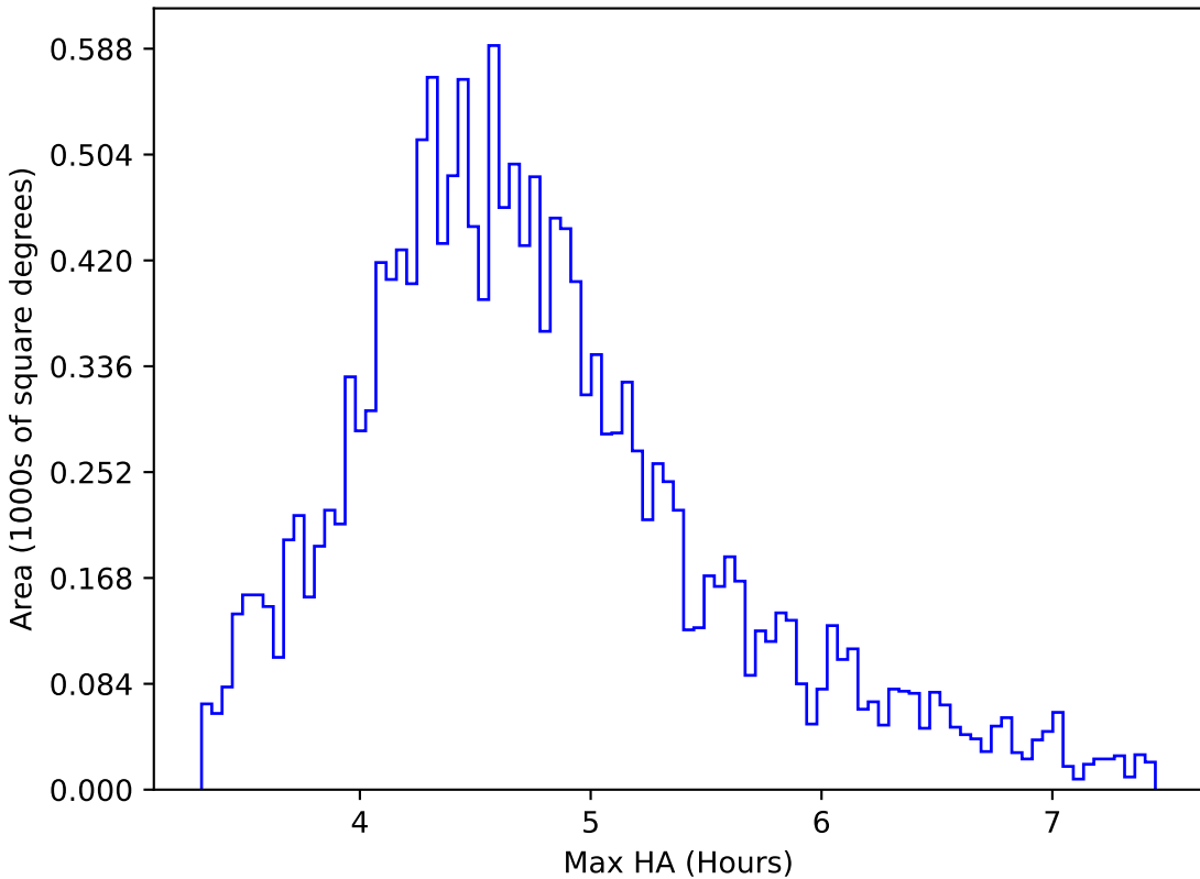
too_elab_r64_d2_gz_v3.4_10yrs WFD y band: Max HA
