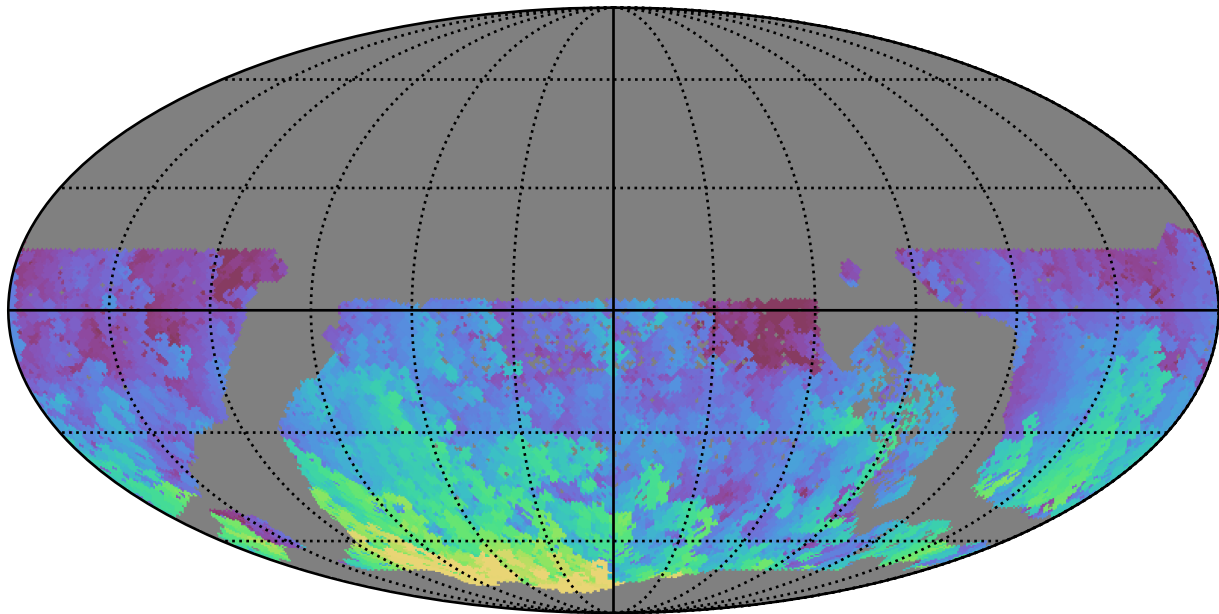
too_elab_r64_d2_gz_v3.4_10yrs WFD u band: Max HA
