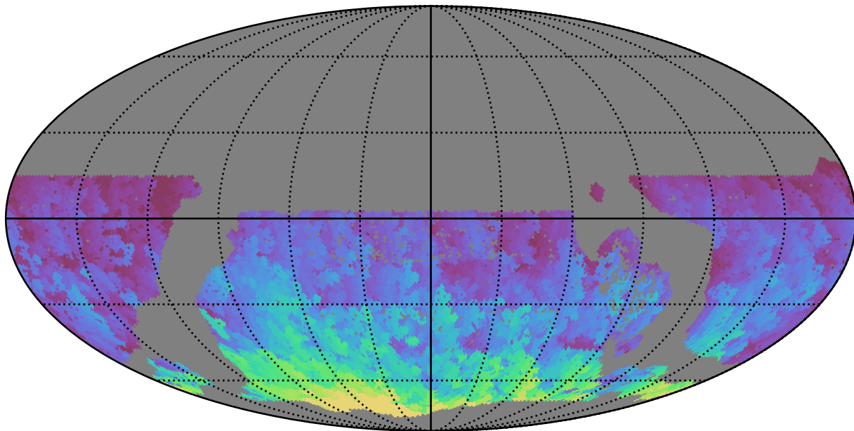
too_elab_r64_d2_gz_v3.4_10yrs WFD r band: Max HA
