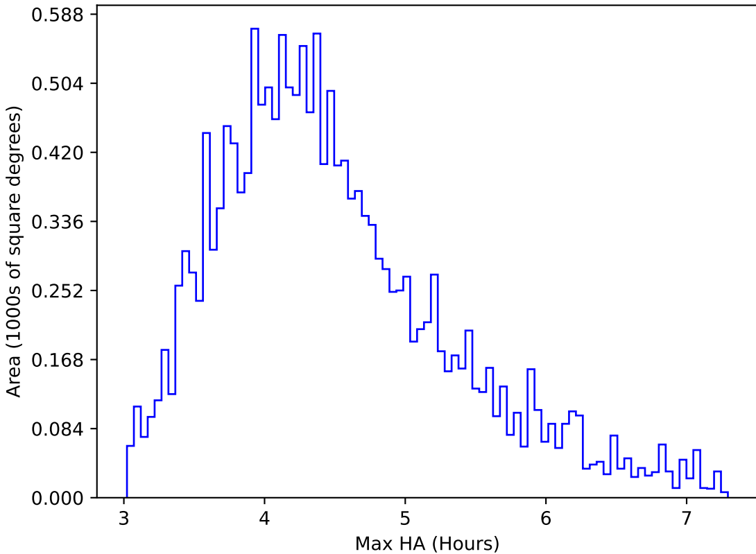
too_elab_r64_d2_gz_v3.4_10yrs WFD r band: Max HA
