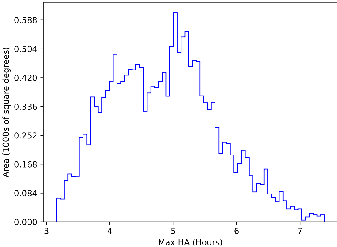
too_elab_r64_d2_gz_v3.4_10yrs WFD i band: Max HA
