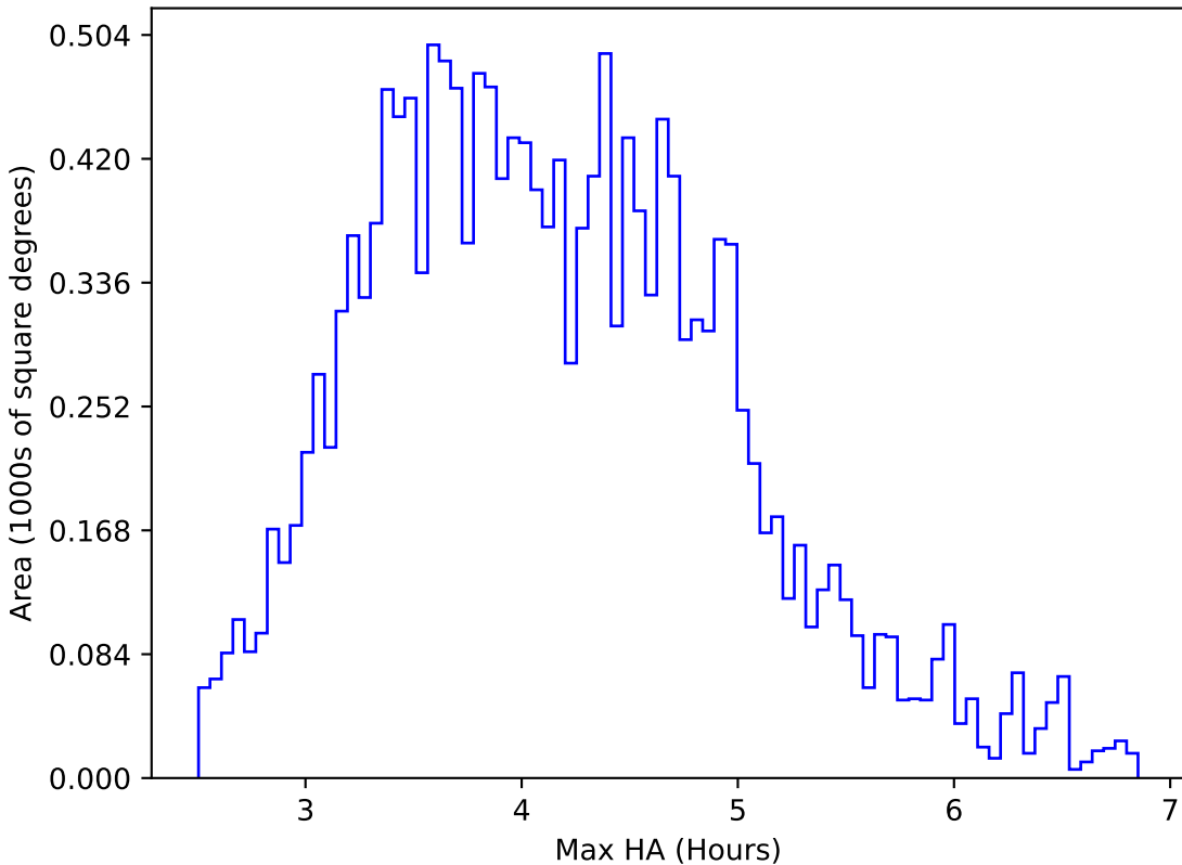
too_elab_r64_d2_gz_v3.4_10yrs WFD g band: Max HA
