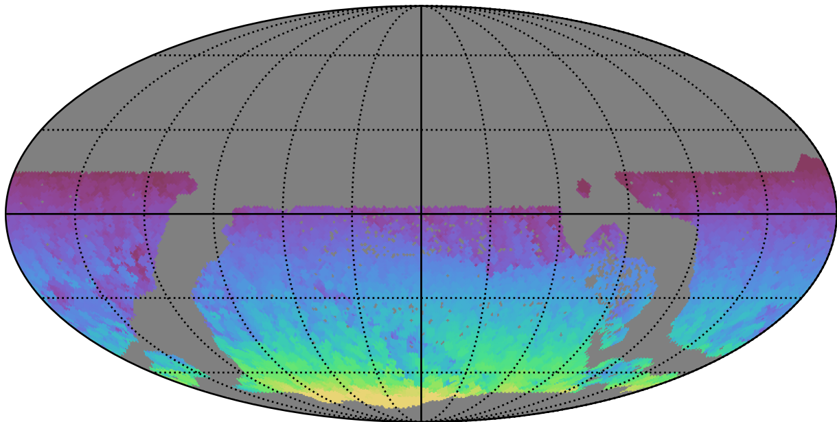
too_elab_r64_d2_gz_v3.4_10yrs WFD all bands: Max HA
