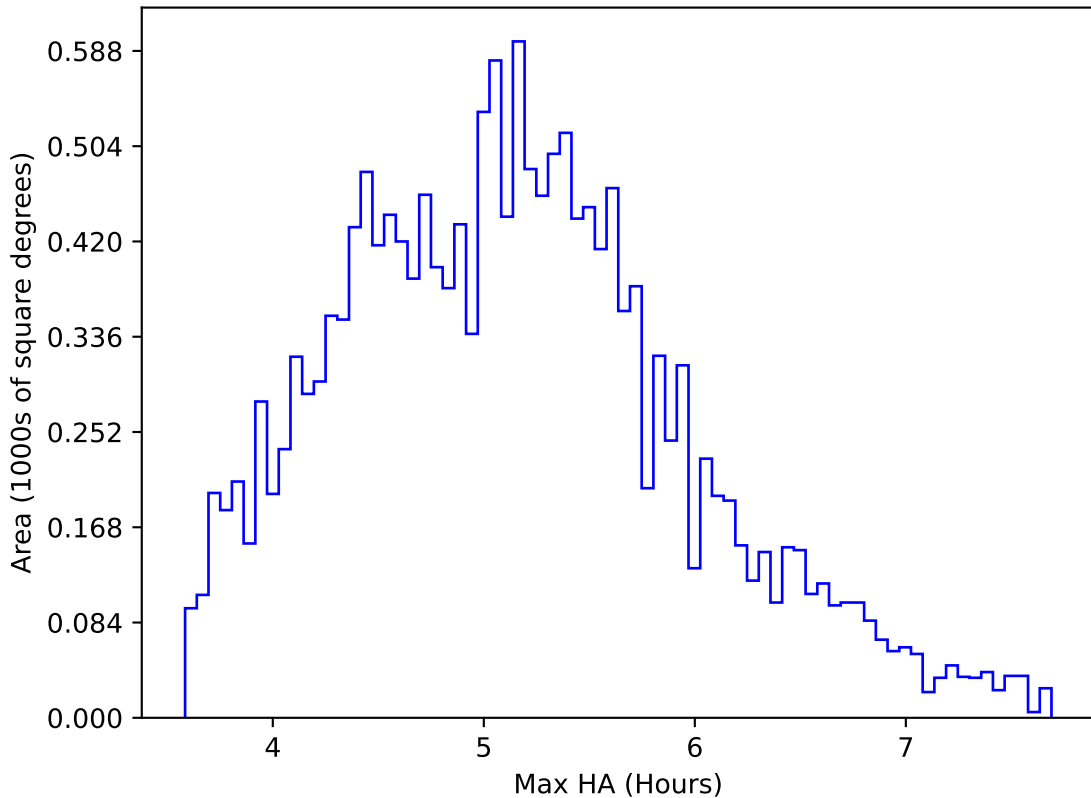
too_elab_r64_d2_gz_v3.4_10yrs WFD all bands: Max HA
