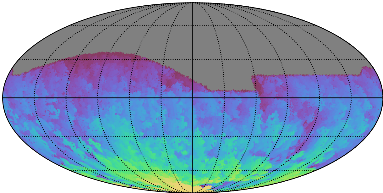
too_elab_r64_d2_gz_v3.4_10yrs All sky r band: Max HA
