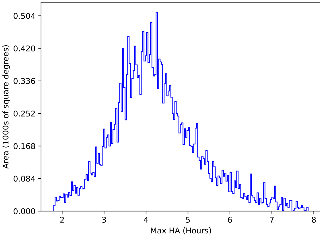
too_elab_r64_d2_gz_v3.4_10yrs All sky r band: Max HA
