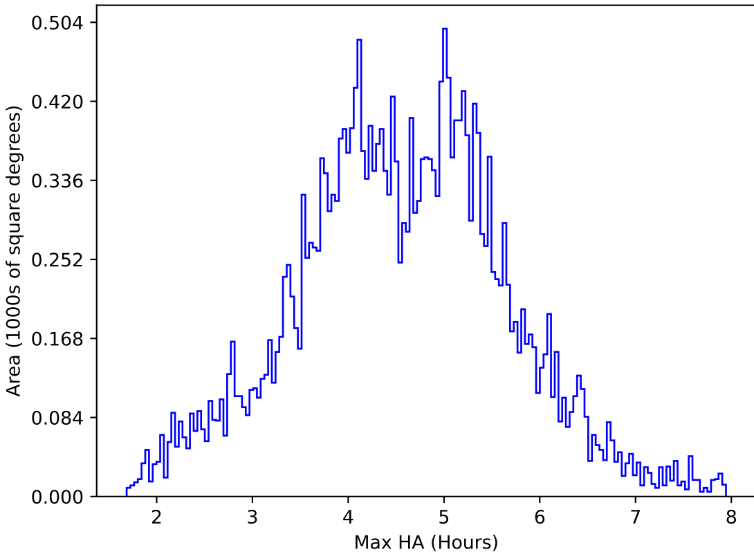
too_elab_r64_d2_gz_v3.4_10yrs All sky i band: Max HA
