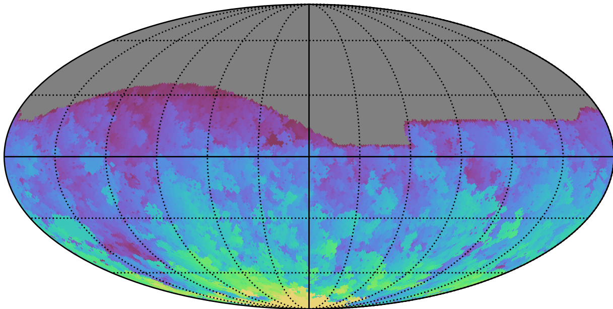
too_elab_r64_d2_gz_v3.4_10yrs All sky g band: Max HA
