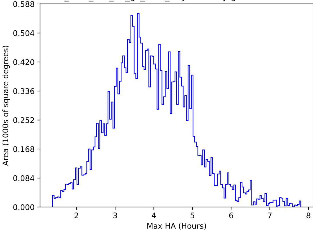
too_elab_r64_d2_gz_v3.4_10yrs All sky g band: Max HA
