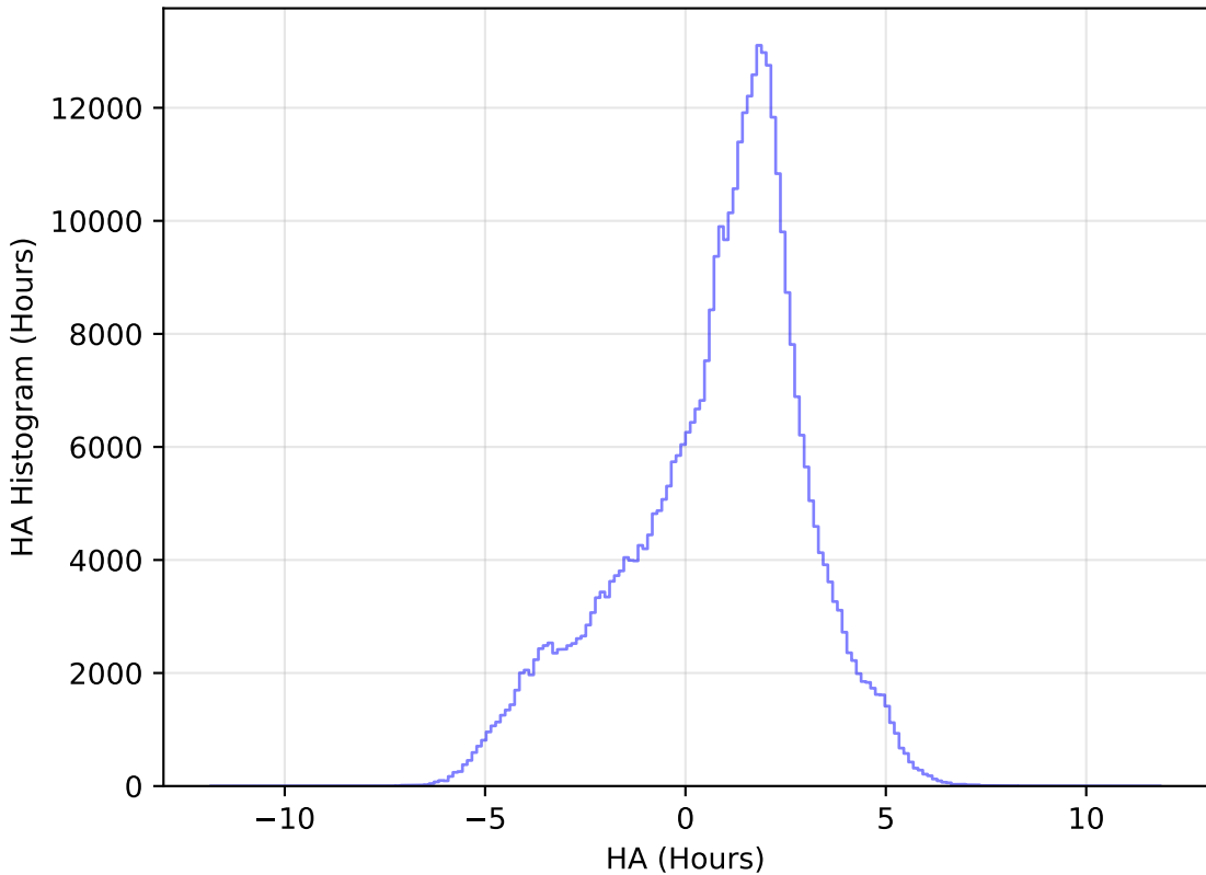
too_elab_r64_d2_gz_v3.4_10yrs WFD z band: HA Histogram
