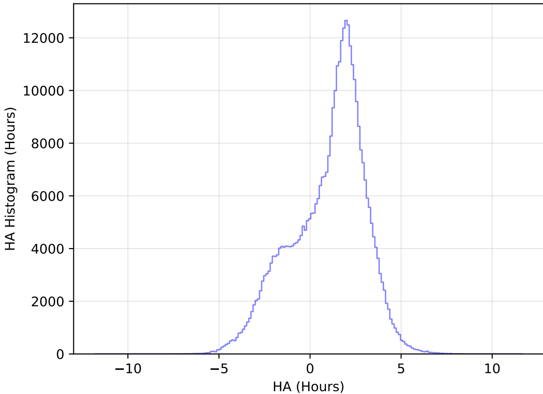
too_elab_r64_d2_gz_v3.4_10yrs WFD y band: HA Histogram
