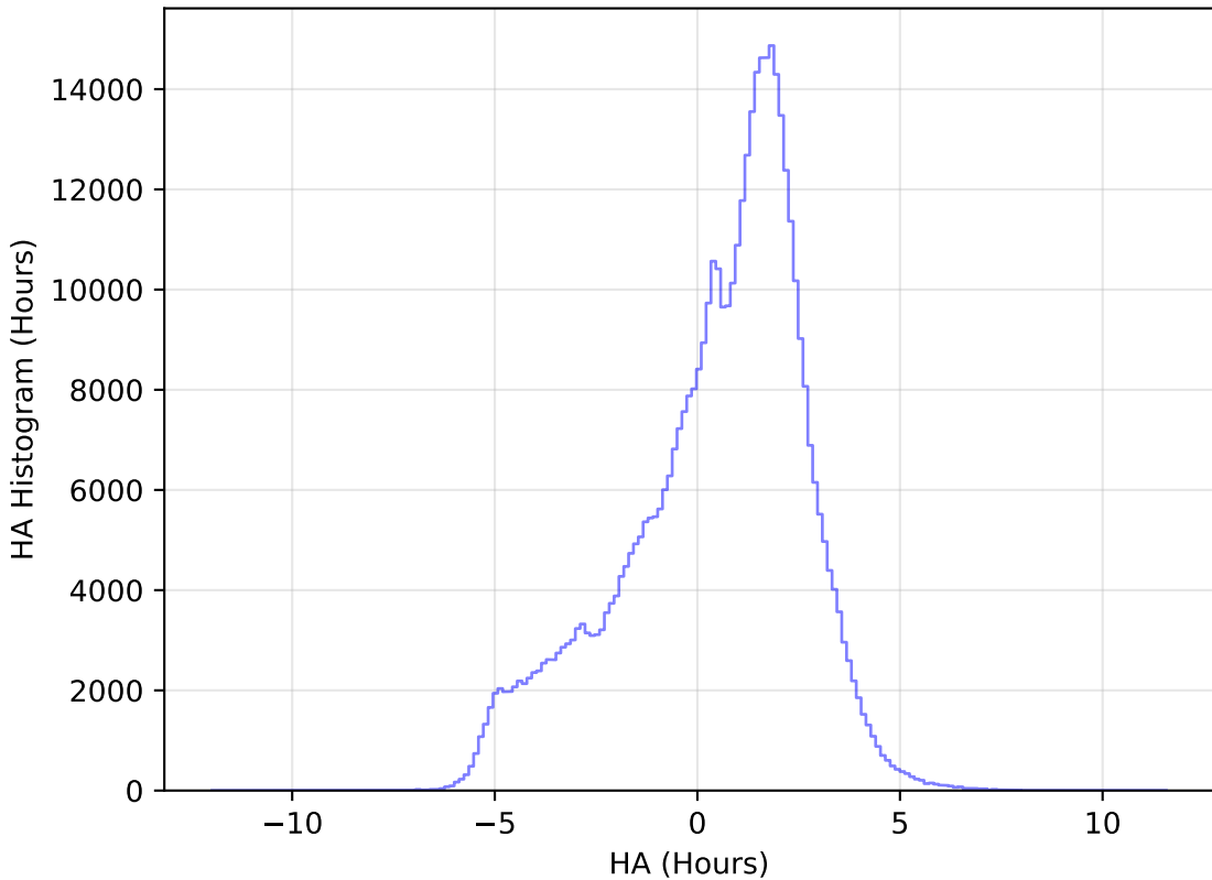
too_elab_r64_d2_gz_v3.4_10yrs WFD r band: HA Histogram
