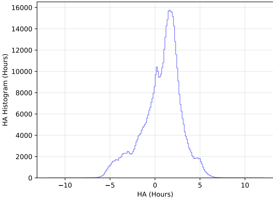
too_elab_r64_d2_gz_v3.4_10yrs WFD i band: HA Histogram
