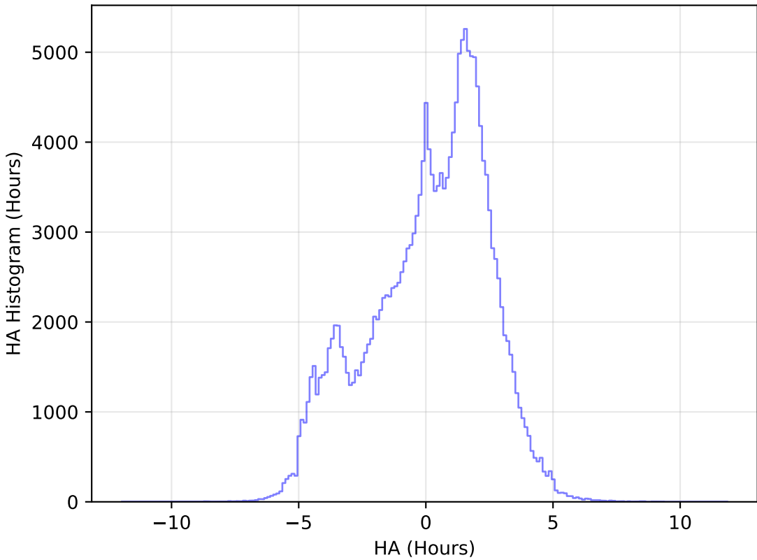
too_elab_r64_d2_gz_v3.4_10yrs WFD g band: HA Histogram
