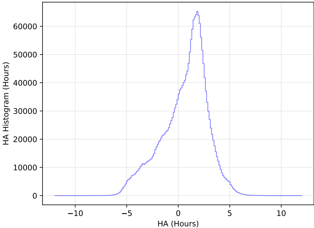
too_elab_r64_d2_gz_v3.4_10yrs WFD all bands: HA Histogram
