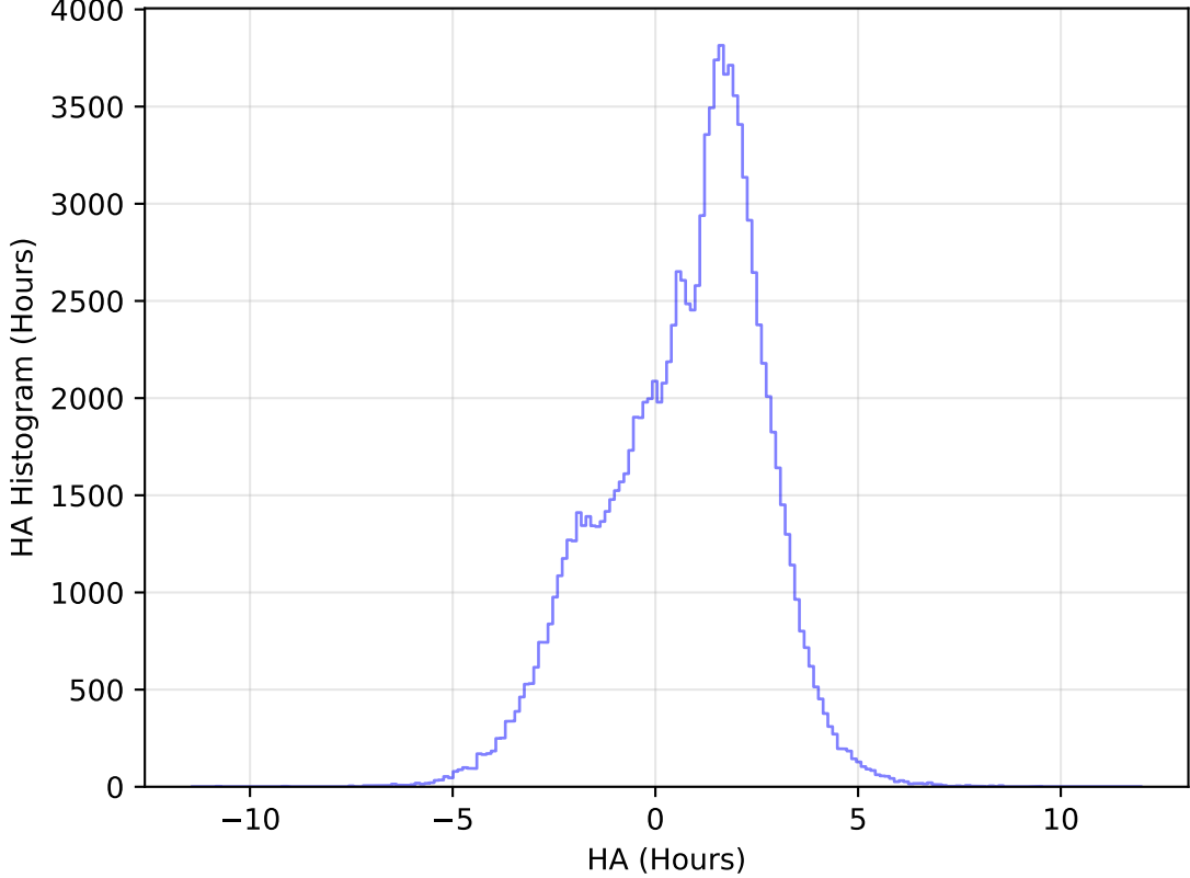
too_elab_r64_d2_gz_v3.4_10yrs All sky u band: HA Histogram
